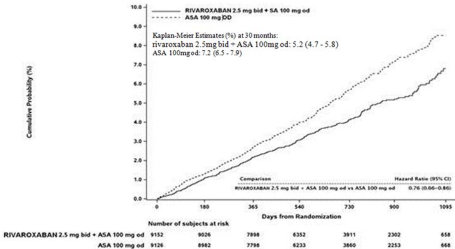
Figure 2: Time to first occurrence of primary efficacy outcome (stroke, myocardial infarction, cardiovascular death) in COMPASS
